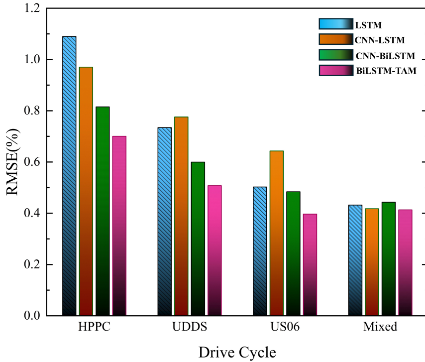
Figure 7: Comparison of RMSE values for different models across various drive cycles (HPPC, UDDS, US06, and Mixed) at 25°C.
