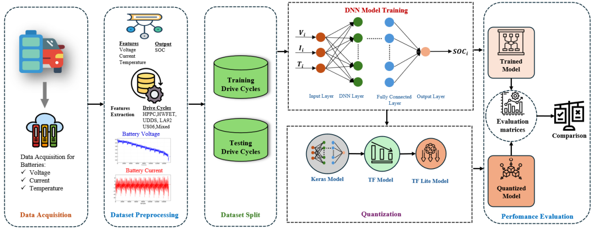
Figure 1: Graphical abstract of SOC estimation using Deep Learning Model with quantisation.
