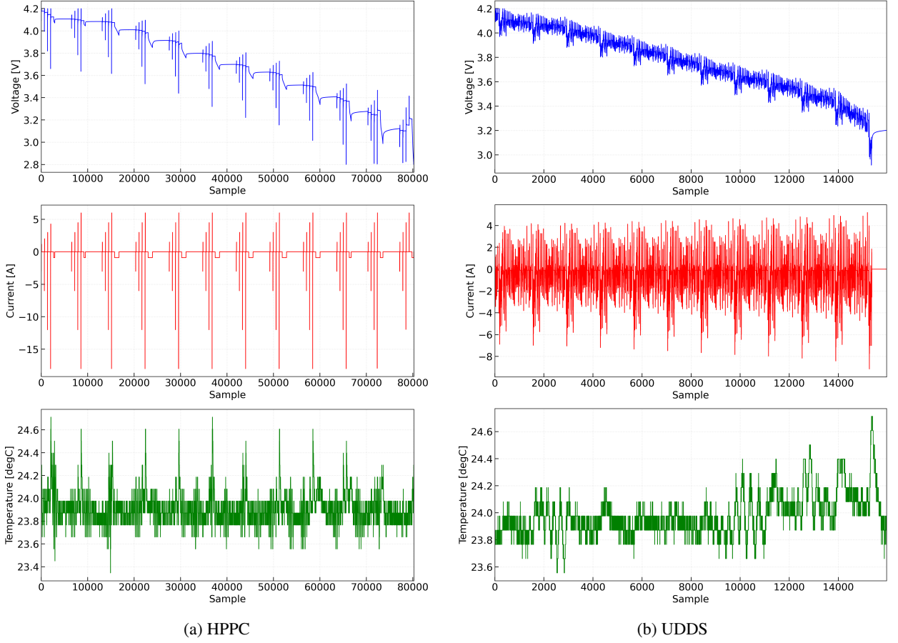
Figure 2: Voltage, current, and temperature variations during the (a)HPPC cycle ,(b) UDDS cycle at 25°C.
