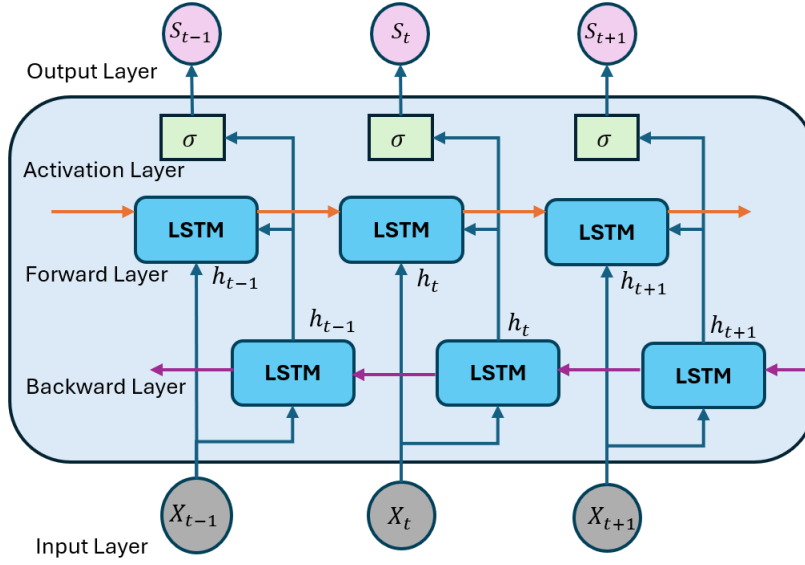
Figure 4: Structure of a BiLSTM cell.
