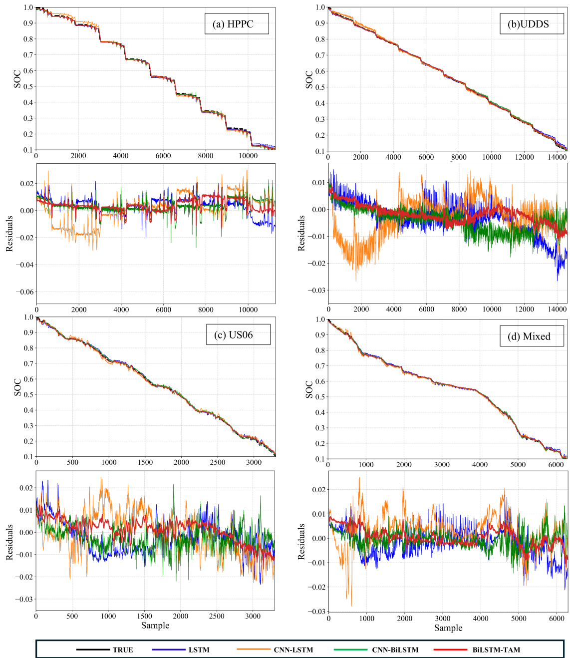
Figure 8: State of Charge (SOC) estimation using four different model at 25°C for different drive cycles: (a) HPPC, (b) UDDS, (c) US06, and (d) Mixed. The top plots in each subfigure show the comparison between the estimated SOC and the true SOC over time (sample index). The bottom plots display the corresponding residuals, representing the difference between the estimated and true SOC values.
