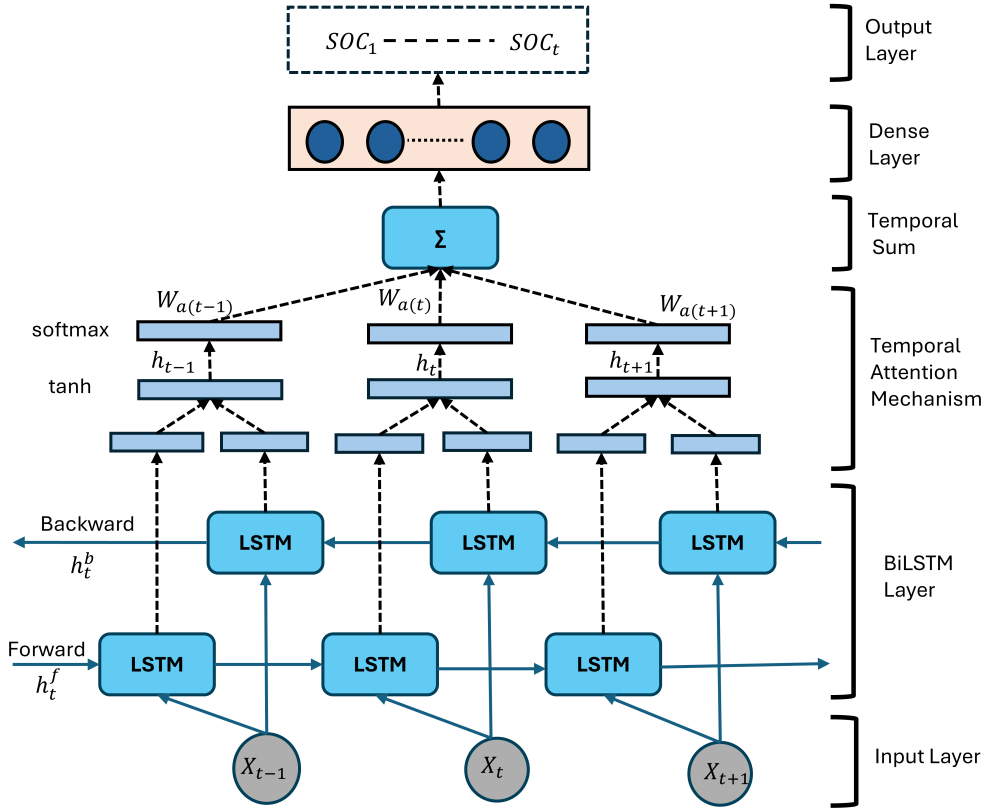
Figure 6: Structure of the Proposed BiLSTM temporal attention mechanism based Algorithm
