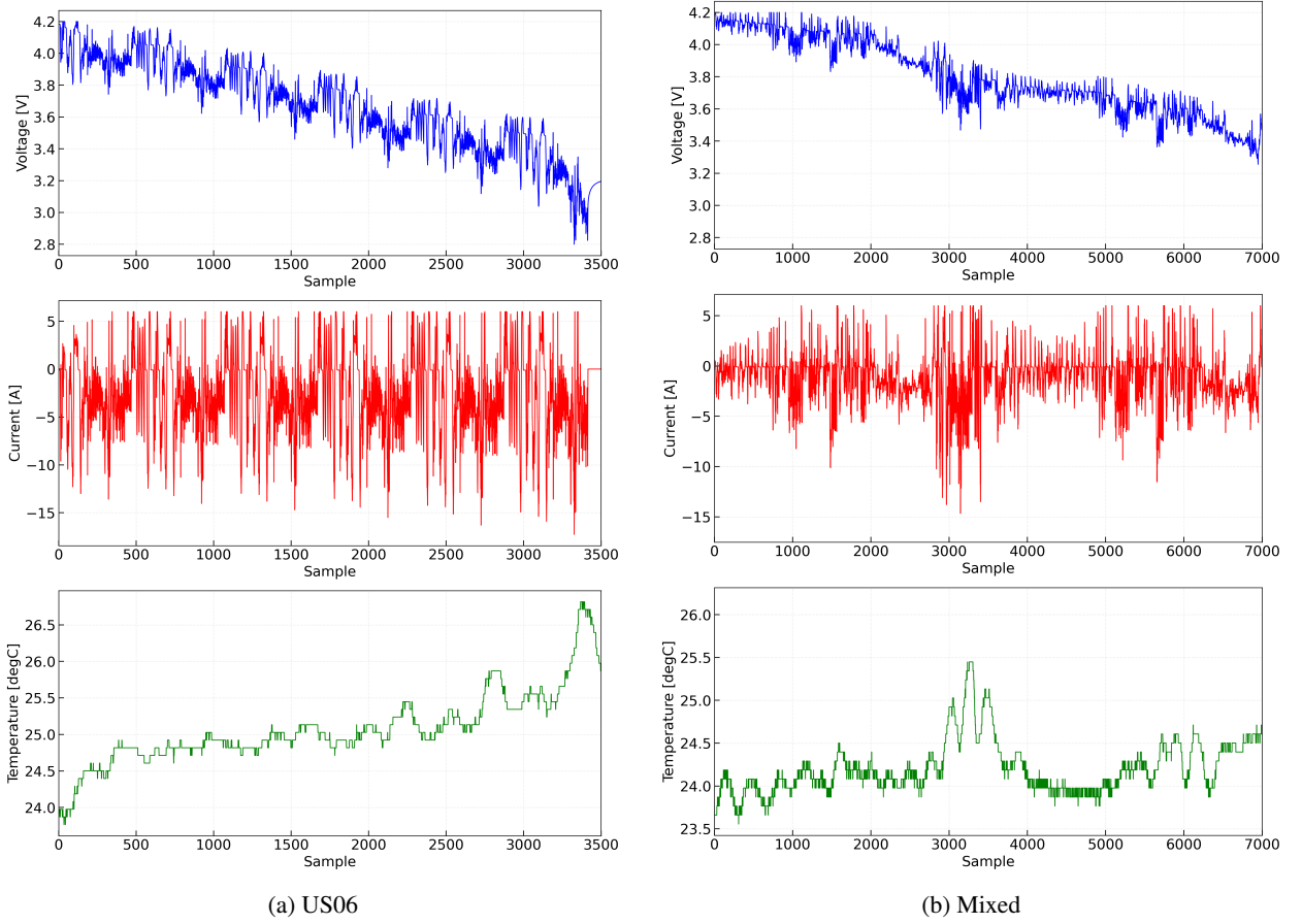
Figure 3: Voltage, current, and temperature variations during the (a)US06 cycle ,(b) Mixed cycle at 25°C.
