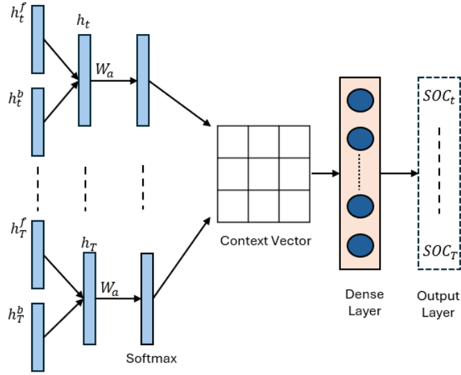
Figure 5: Structure of Temporal Attention Mechanism to estimate the SOC at each time step.
