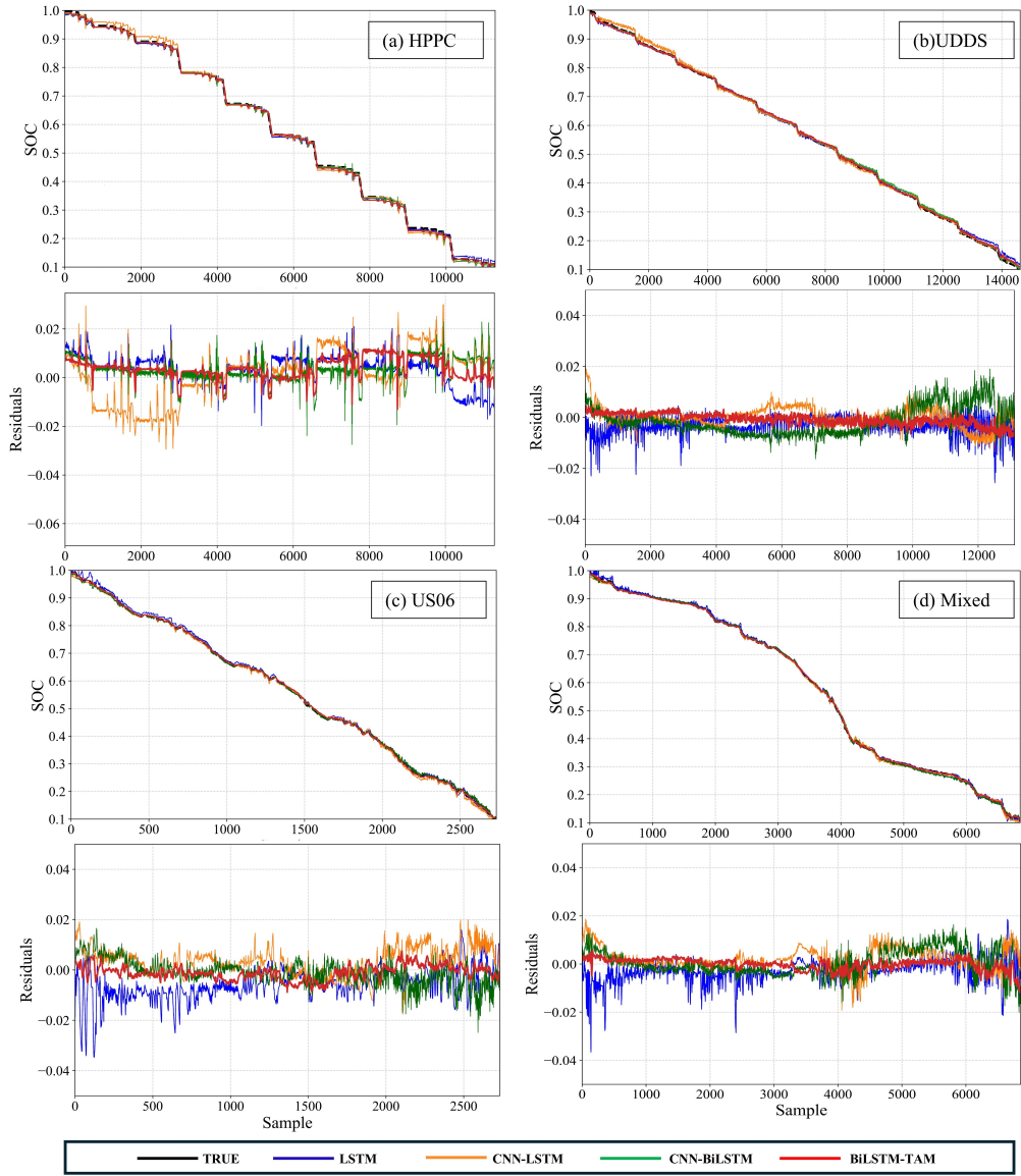
Figure 9: State of Charge (SOC) estimation using four different model at 0°C for different drive cycles: (a) HPPC, (b) UDDS, (c) US06, and (d) Mixed. The top plots in each subfigure show the comparison between the estimated SOC and the true SOC over time (sample index). The bottom plots display the corresponding residuals, representing the difference between the estimated and true SOC values.
