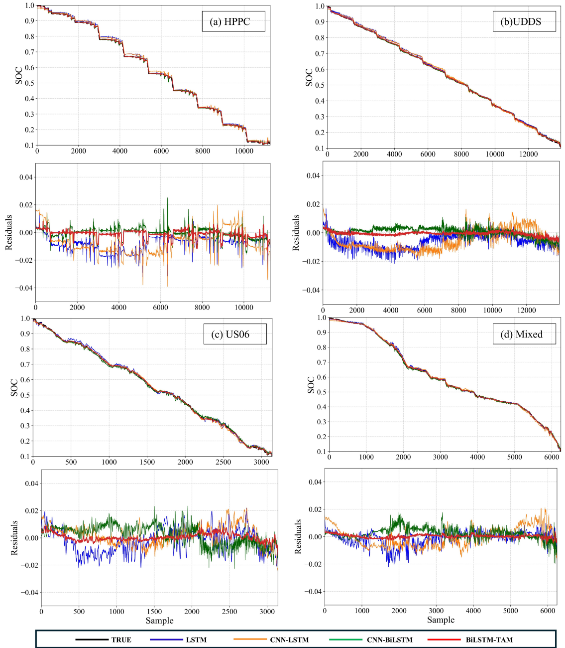
Figure 10: State of Charge (SOC) estimation using four different model at 10°C for different drive cycles: (a) HPPC, (b) UDDS, (c) US06, and (d) Mixed. The top plots in each subfigure show the comparison between the estimated SOC and the true SOC over time (sample index). The bottom plots display the corresponding residuals, representing the difference between the estimated and true SOC values.
